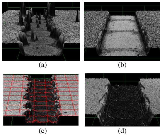
Figure 9: Microscope images of a a) P2 scribe using a 20 \mu\text{m} Gaussian beam and b) P3 scribe using a 37 \mu\text{m} square-beam profile (3D confocal microscope image), both on CdTe PV devices. 3D images of a c) Gaussian beam P3 scribe and d) a square beam P2 scribe of a-Si, both acquired using a confocal laser microscope.
