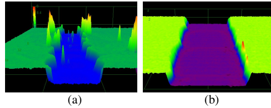
Figure 10: Confocal laser microscope 3D images of P3 scribes in CdTe using (a) a Gaussian beam and (b) a square flat-top shaped beam.
