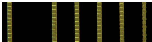
Figure 6: Transmission microphotograph of P2 scribes on CdTe with the square-beam shaping apparatus. Single pulses were used to scribe the individual squares, at a speed of 7000 \text{ mm/s} , with laser pulse repetition rate of 200 \text{ kHz} and fluences from 0.11\text{-}0.23 \text{ J/cm}^2 (right to left).
