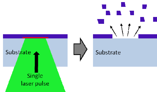
Figure 5: Diagram of a backside processing (superstrate, or lift-off) geometry. A single laser pulse ablates a small volume of material but results in removal of a much larger volume.
