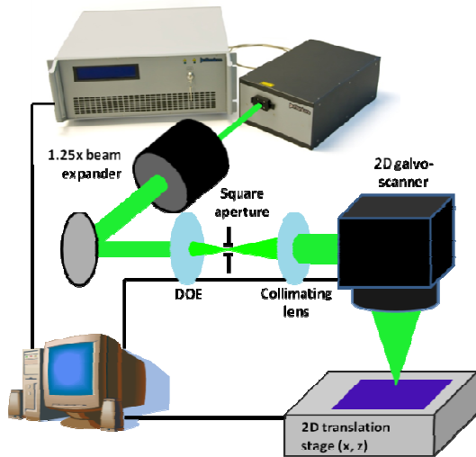
Figure 1: Schematic of the beam-shaping apparatus. DOE denotes the HoloOr flat-top beam shaper.
