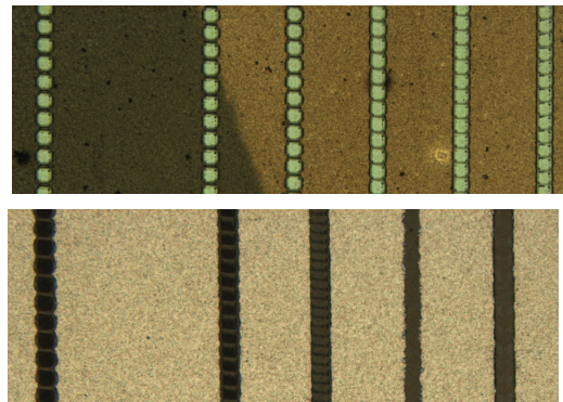
Figure 8: Reflection microphotograph of and P3 CdTe scribes (top) and P2 a-Si (bottom) with the square-beam shaping apparatus. Single pulses were used to scribe the CdTe (top), at speeds of 6000\text{-}9000 \text{ mm/s} (right to left). The P2 a-Si was scribed at speeds of 1000\text{-}8000 \text{ mm/s} (right to left), with laser pulse repetition rate of 200 \text{ kHz} and fluence of 0.205 \text{ J/cm}^2 .
