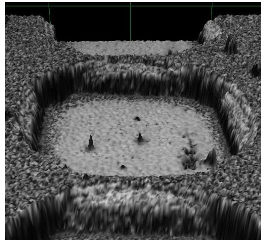
Figure 4: Square removal area created from a very high speed P3 scribe of a CdTe PV device utilizing a square flat-top shaped processing beam.
