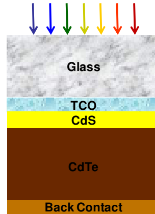
Figure 3: CdTe photovoltaic device construction.
