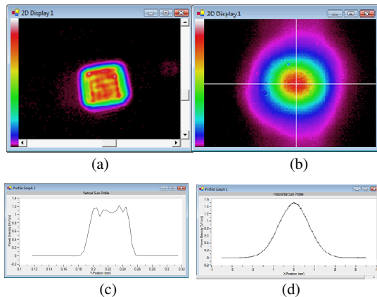
Figure 2: Typical 2D profiles of a) spatially shaped square beam and b) Gaussian beam employed in the present work. The profiles for the square and Gaussian beams are shown in (c) and (d) respectively.
