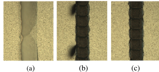
Figure 7: Reflection microphotographs of P3 scribes on a-Si with the square-beam shaping apparatus. Picosecond laser pulses at a repetition rate of 200 \text{ kHz} were used to scribe the squares, at a speed of 7000 \text{ mm/s} , and with fluences of a) 0.16 , b) 0.18 and c) 0.23 \text{ J/cm}^2 .
